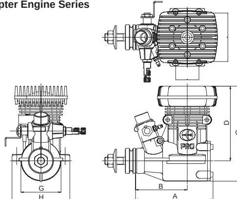
Helicopter Engine Series
