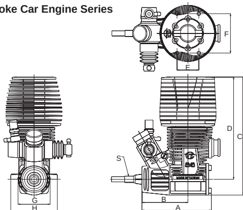
Two-Stroke Car Engine Series
