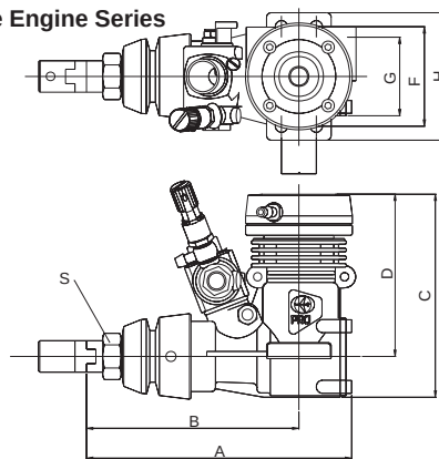
Two-Stroke Marine Engine Series
