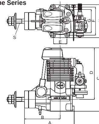
Four Stroke Engine Series
